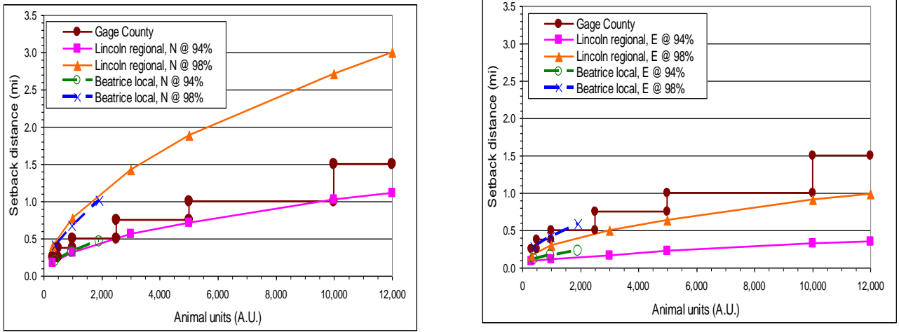
Figure B1. Setback distances as specified in Gage County zoning ordinances and as given by odor footprint modeling for various sizes of deep-pit swine finishing facilities for the a) worst-case, north direction (left) and b) best-case, east direction (right).
