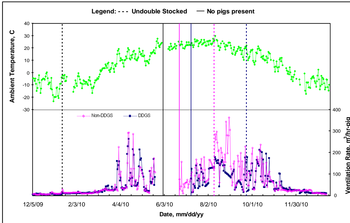
Figure 2. Average ventilation rate ( \text{m}^3 \text{hr}^{-1} \text{pig}^{-1} ) for each barn and ambient temperature.
